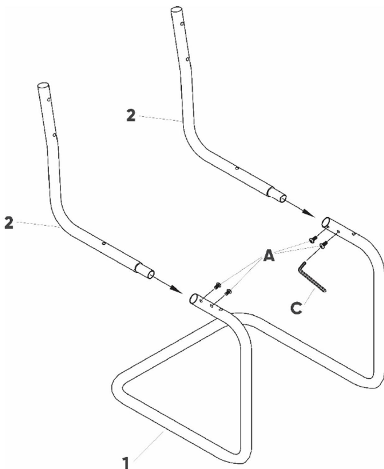
C Allen key (x1)
